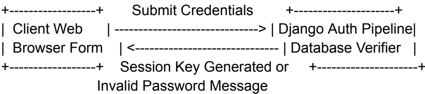
Diagram 4.1: Login Flow Diagram
