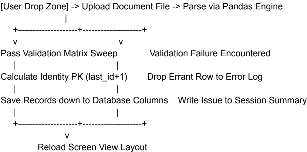
Diagram 9.1: Excel Sheet Processing Pipeline Runbook Flow
