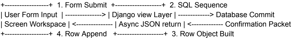
Diagram 7.1: Fetch API Ingestion Matrix Map
